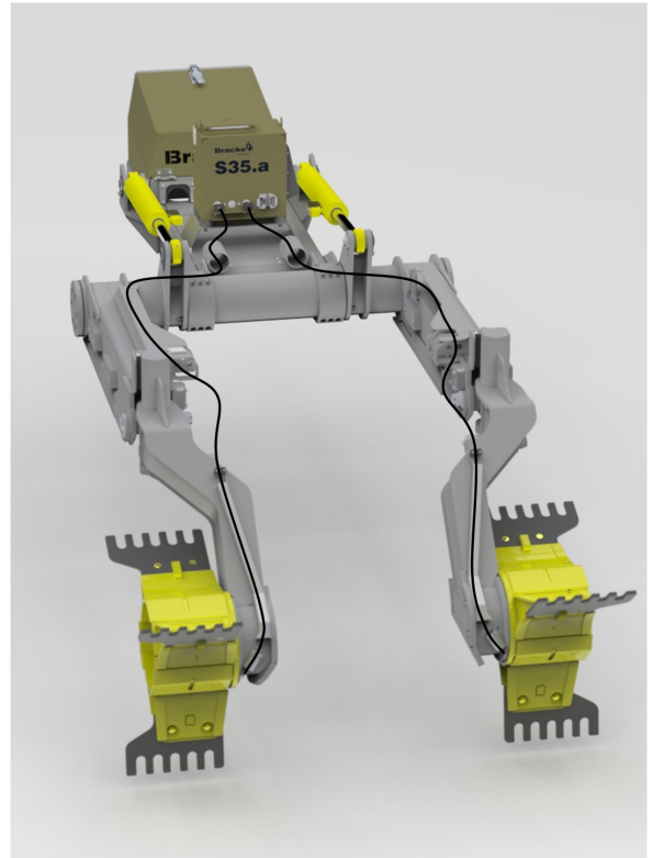
The Bracke S35.a attaches to a scarifier and the seeds are fed through a tube to the seedbed. Individual seed feed wheels control the flow of seeds to each sowing channel.
